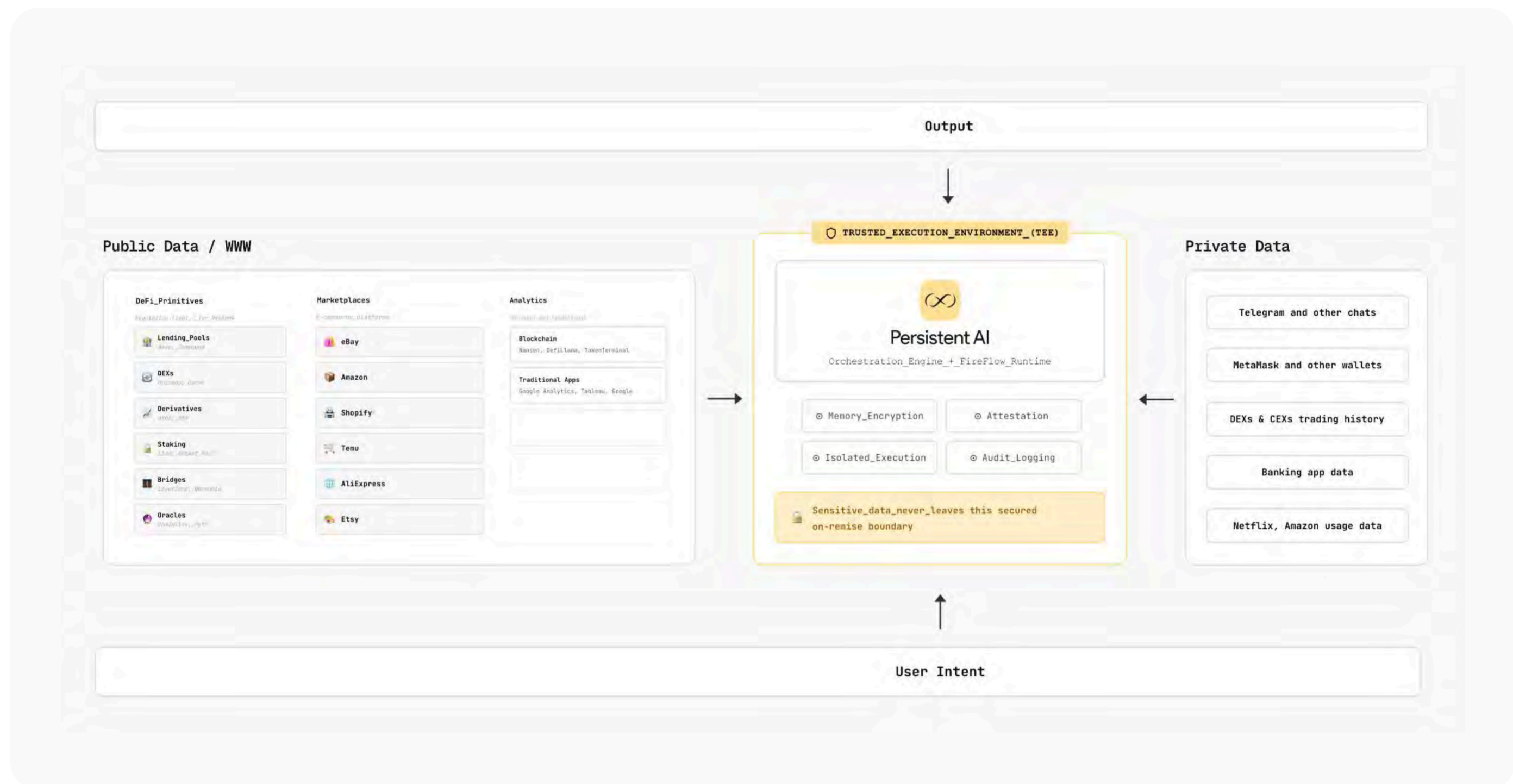
Fig13: Orchestration Layer
