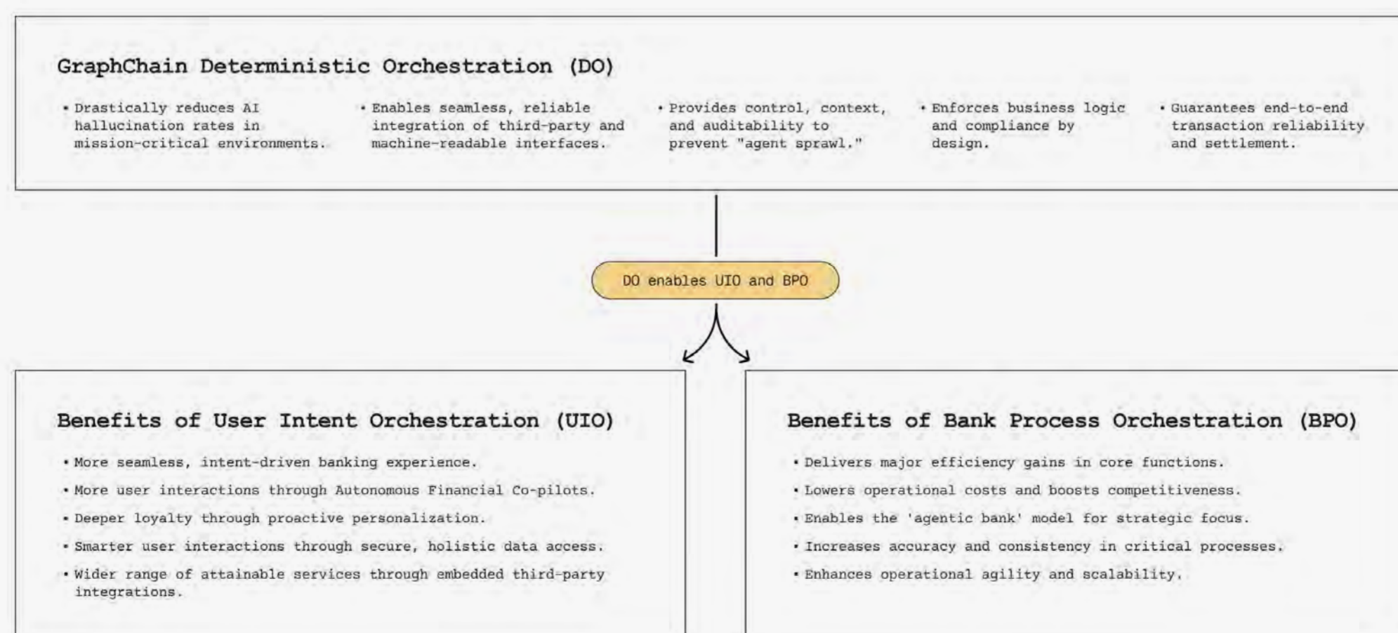
Fig3: Deterministic Orchestration
