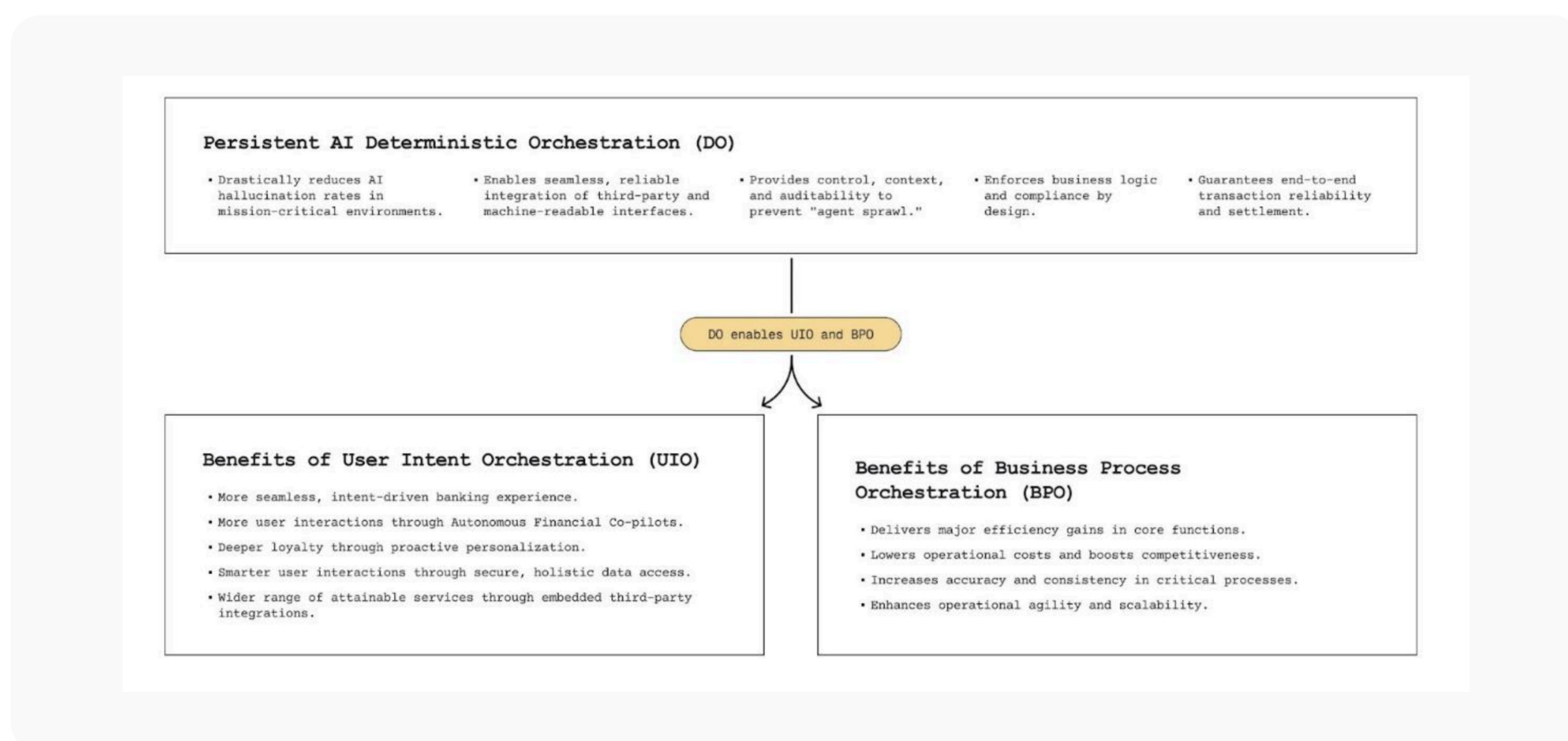
Fig14: Deterministic Orchestration
